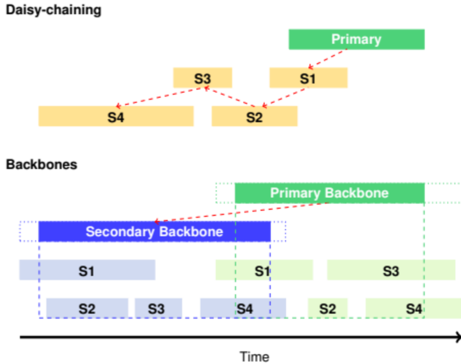
Figure 10. Schematic showing the difference between daisy-chaining and backbone methodologies. In daisy chaining, primary (green) and secondary observers (tan) are scaled sequentially to each other based on their interval of overlap. In the backbone method (Svalgaard and Schatten, 2016), several secondary observers (light-green and light-blue) are scaled to multiple backbone observers based on their interval of overlap and then the contiguous backbone series tied to each primary observer are scaled to each other. While both daisy-chaining (e.g., Hoyt and Schatten, 1998a,b) and the backbone method employ daisy-chaining, the advantage of the backbone method is the reduction of the number of links in the chain, reducing the accumulation of errors. See text for differences in the backbone approach employed by Svalgaard and Schatten (2016) and Chatzistergos et al. (2017). (Adapted from Chatzistergos, 2017.)
